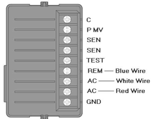
Simple Three Wire Installation
